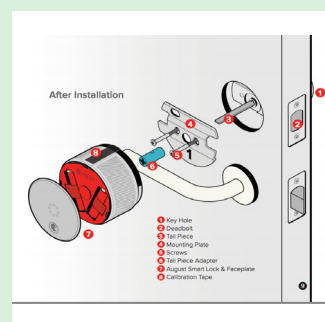
10. Component Diagram 1
