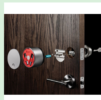
11. Component Diagram 2
